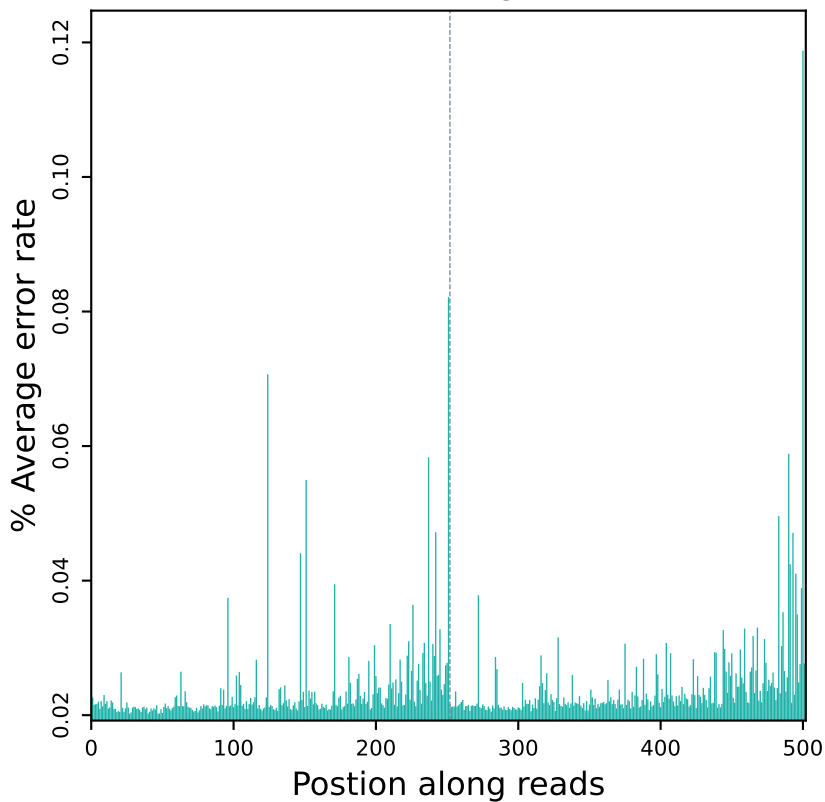
Error rate distribution along reads (R10610)
